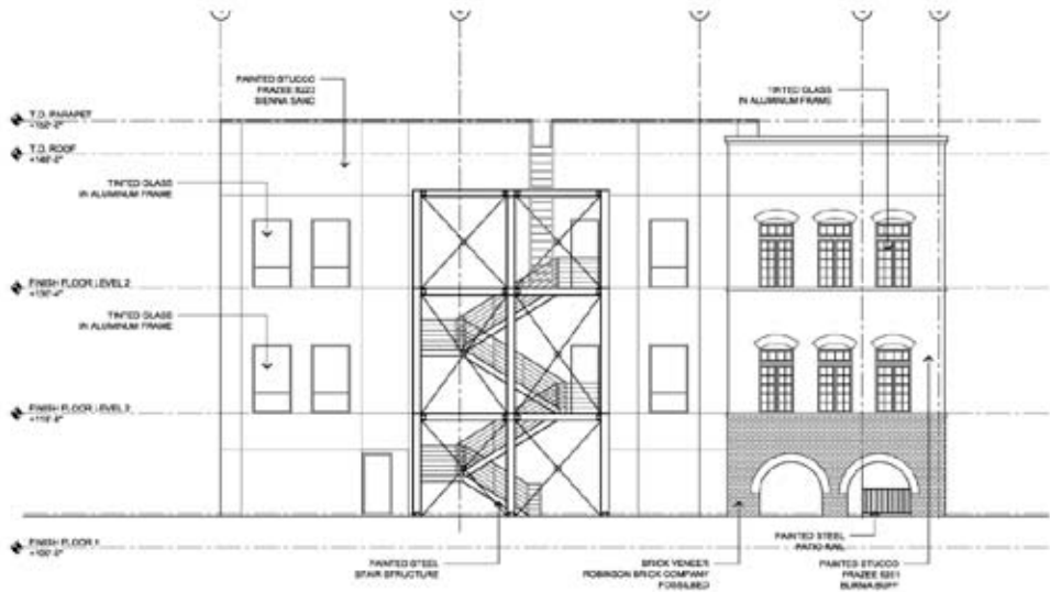
WEST ELEVATION
