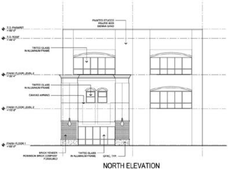
NORTH ELEVATION
