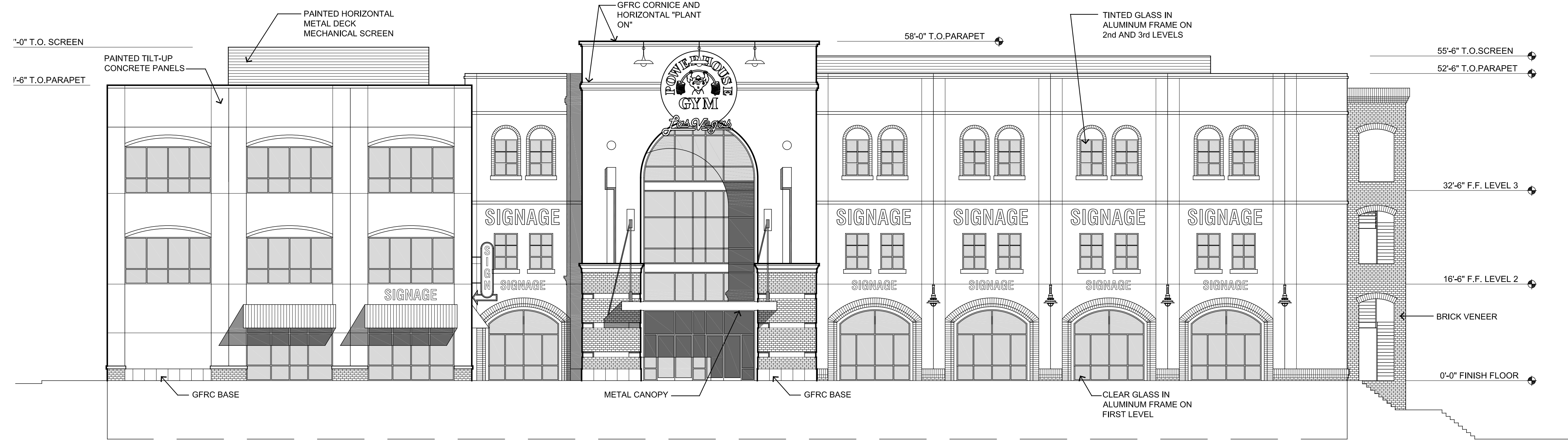
SOUTH ELEVATION
